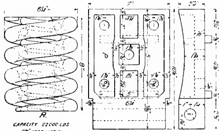
Fig. 5525. DRAFT-SPRING.
